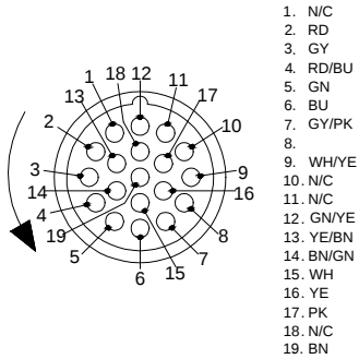
FEMALE END VIEW
